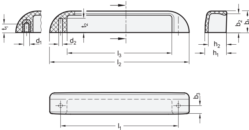
ELESA original design MLP
